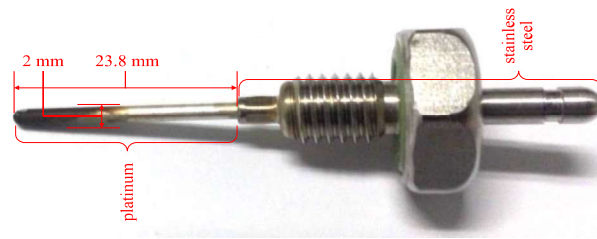
Figure 5. Grading electrodes
