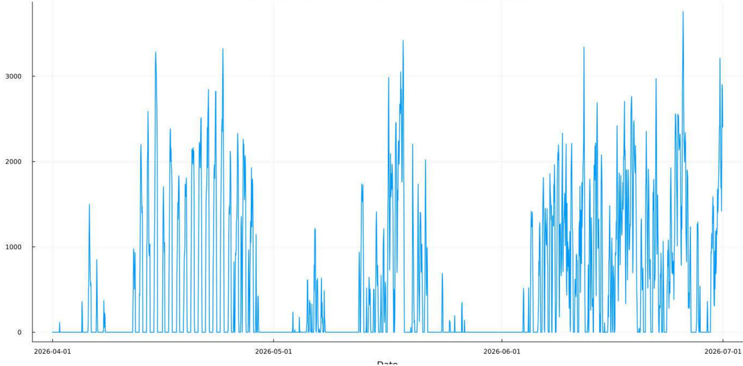
EUE Time-Series - Median_LOLP (EUE_Simulation_134)
