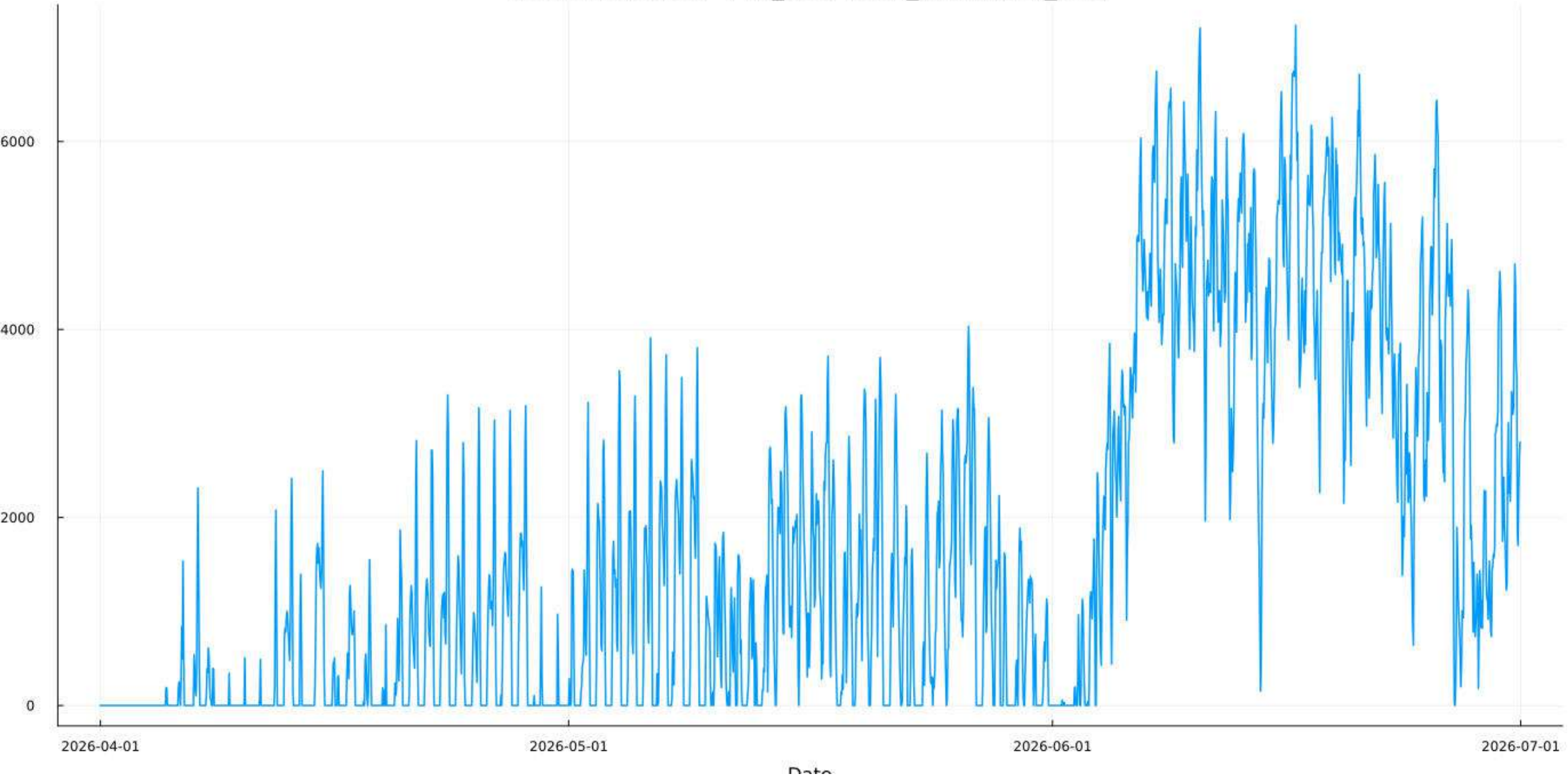
EUE Time-Series - Min_LOLP (EUE_Simulation_936)
