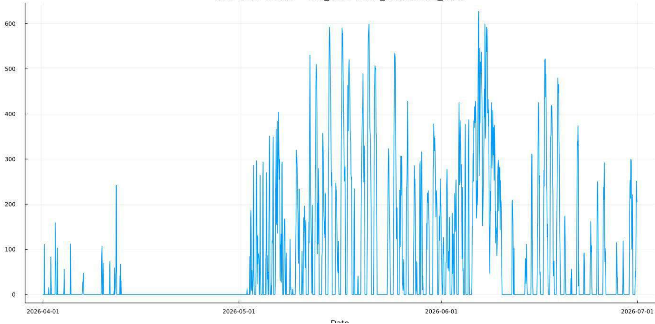
EUE Time-Series - Min_LOLP (EUE_Simulation_692)
