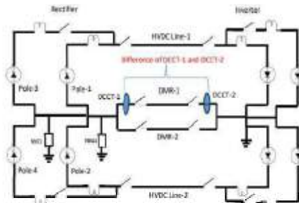
Figure 94: DMR current differential protection
