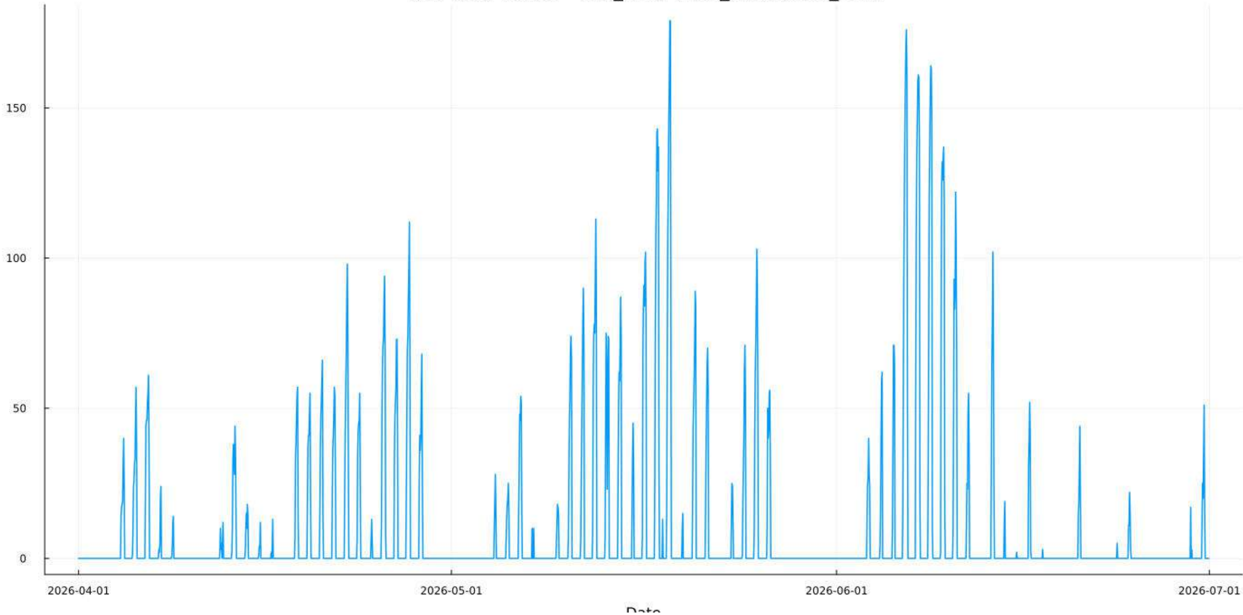
EUE Time-Series - Min_LOLP (EUE_Simulation_144)
