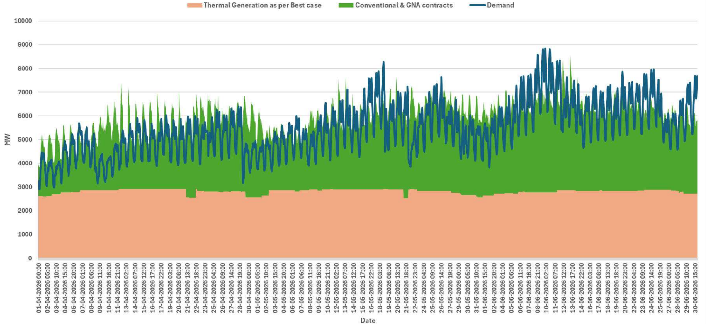
Demand vs Supply Mix (Thermal + Conventional/GNA) for April-June 2026
