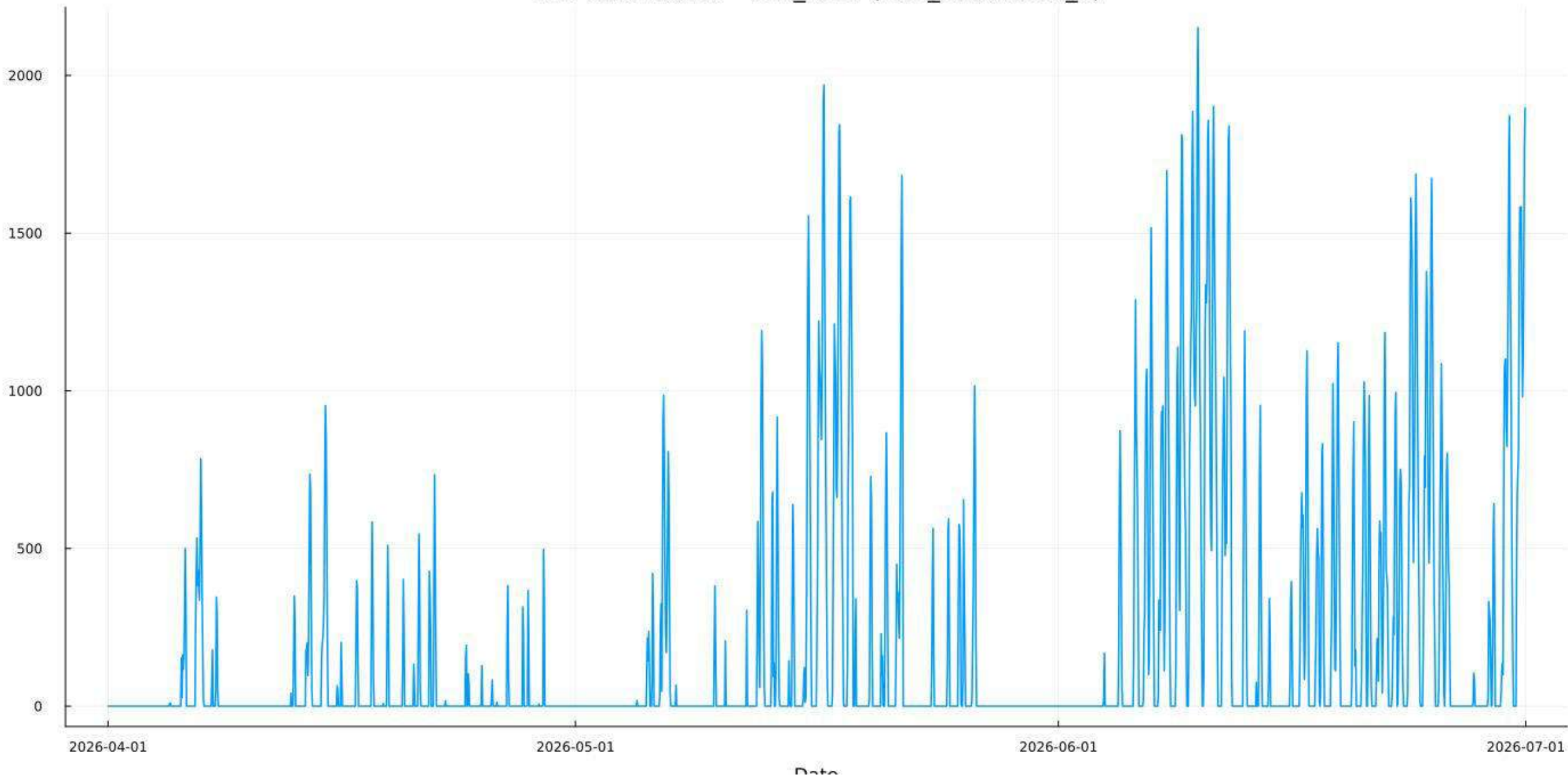
EUE Time-Series - Min_LOLP (EUE_Simulation_5)
